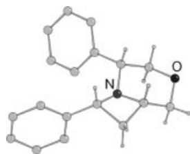
Figure 3. X-ray structure of 5a .
