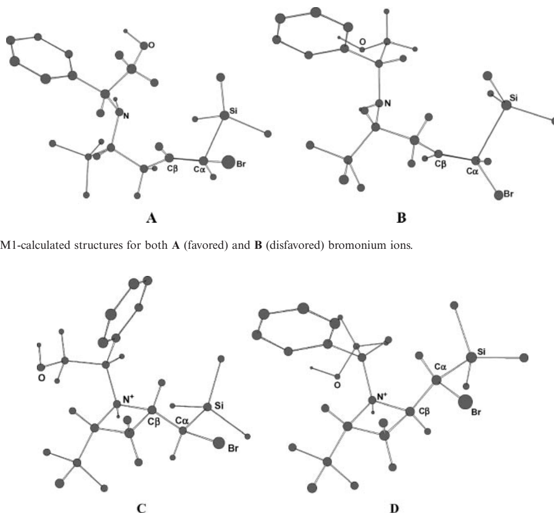
Figure 2. AM1-calculated structures for both C (favored) and D (disfavored) azetidinium ions.
